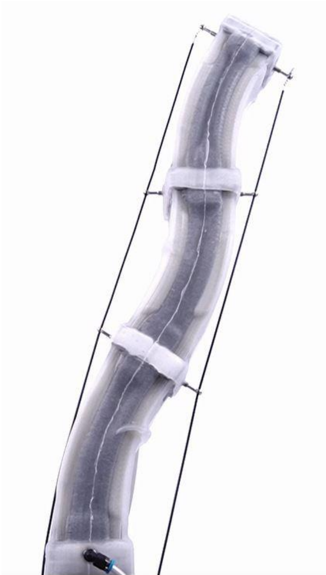
Fig. 2 Current status of the research at Fraunhofer IWU: robot arm consisting of three segments with switchable stiffness and tendons to execute a range of different movements
