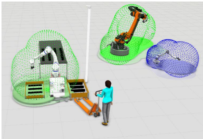
Fig. 1 Modular safety system for the next generation of human-robot collaboration: Developed by Fraunhofer IWU, NexCOBOT and Synapticon © Fraunhofer IWU www.iwu.fraunhofer.de/en.html
